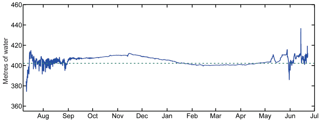
Figure 3-10. Pressure record from borehole GL 11-1C for period July 2011 to late June 2012. Data plotted as m of water equivalent above the bed; full ice thickness is 460 m. Dashed green line shows time-average water pressure for the period of record, and corresponds to 98% of overburden pressure.
