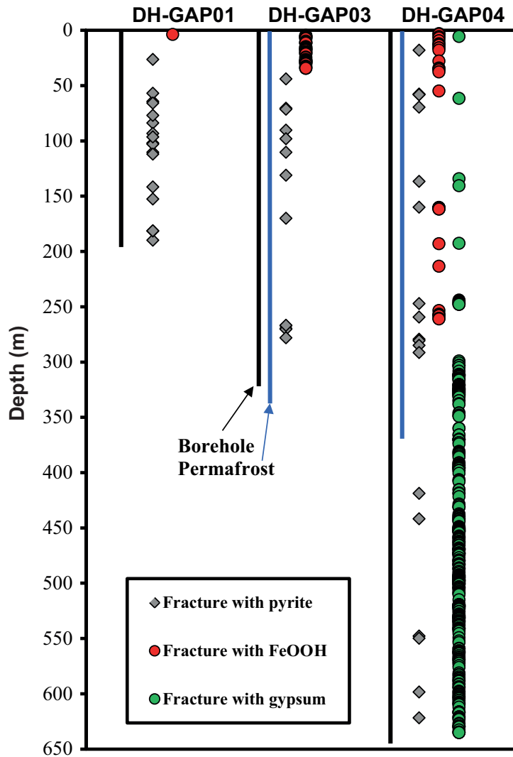
Figure 3-25. Mapping of fracture minerals, goethite ( FeOOH ), pyrite and gypsum vs. depth. On the x-axis, there is one column for each mineral in each of the boreholes. Y-axis shows vertical depth from top of casing (TOC).
