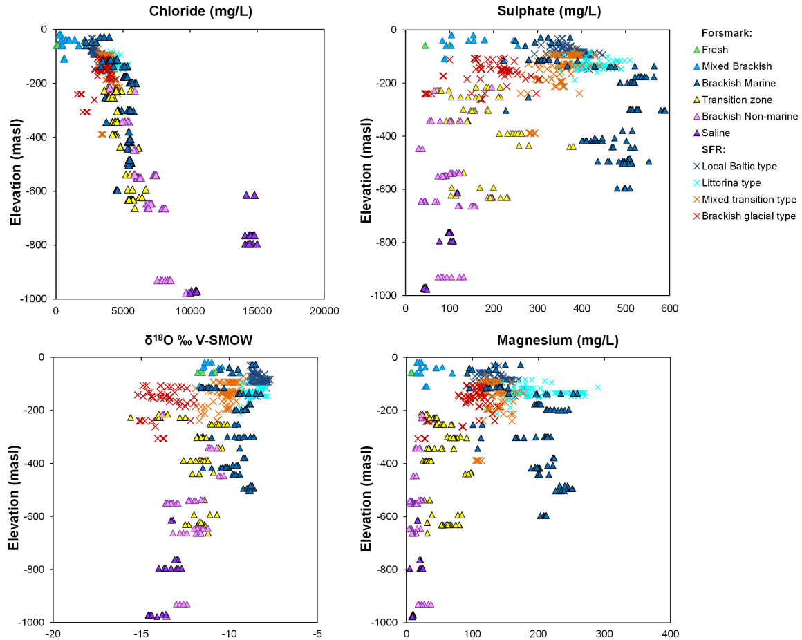
Figure 3-19. Distribution of chloride, sulphate, \delta^{18}\text{O} and magnesium with depth related to the different groundwater types defined for the Forsmark and SFR sites (Laaksoharju et al. 2008b, Nilsson et al. 2011).
