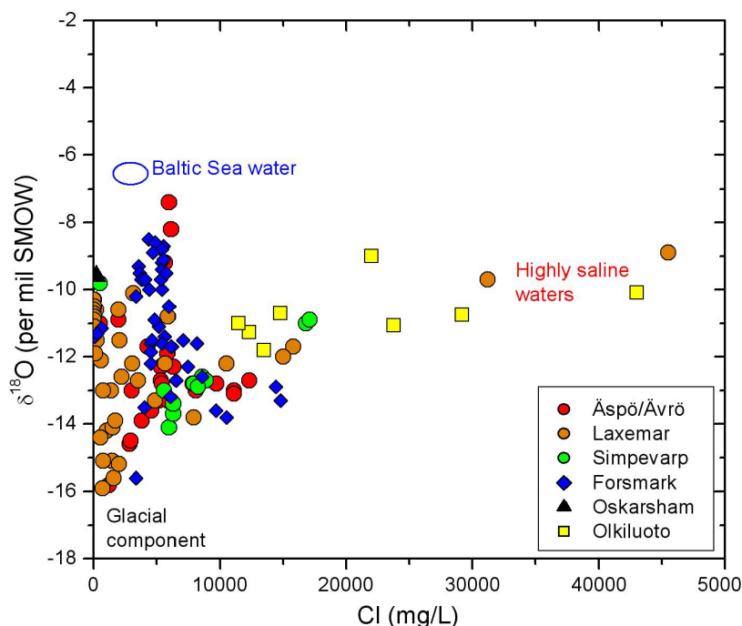
Figure 3-20. \delta^{18}\text{O} versus chloride (categories 1–4) for the most well documented sites around the Baltic (Smellie et al. 2008).
