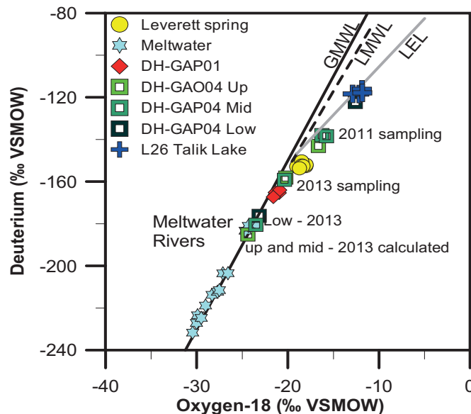
Figure 3-23. \delta^{18}\text{O} versus \delta^2\text{H} for groundwaters, meltwaters and the Talik lake (L26, the lake overlying DH-GAP01). The calculated isotopic composition of DH-GAP04 waters is based on a simple linear mixing model. LEL is the local evaporation line, and LMWL is the local meteoric water line.
