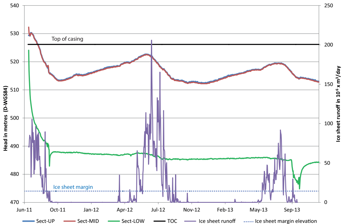
Figure 3-16. Daily average hydraulic heads in Sect-up, Sect-mid and Sect-low in borehole DH-GAP04 and surface meltwater runoff from the Kangerlussuaq sector of the GrIS. Runoff in the figure is represented as total modelled runoff within the delineated surface catchment (for catchment delination see Figure 1-4a and for details see Data Report 2016). Note that the head curves for Sect-up (blue curve) and Sect-mid (red curve) overlie each other. TOC stands for top of casing. The dashed line shows the elevation of the ice sheet margin, indicating that pressure levels in the borehole are artesian. Successful water sampling campaigns were carried out in all sections in September 2011 and 2013.
