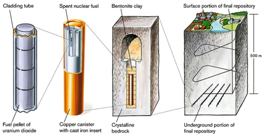
Figure 3.1-1. SKB's KBS-3V concept (SKB 2010).
