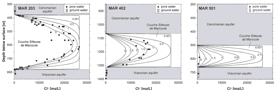
Figure 6.3.2-3. Base-case model (runs G203 A5, G402 A5, G501 A5 are shown) for the out-diffusion of \text{Cl}^- in the Couche Silteuse de Marcoule considering an initial concentration of 25,900 \text{ mg L}^{-1} (the maximum observed \text{Cl}^- concentration in the Couche Silteuse – see Figure 6.3.2-2). Values adjacent to model curves indicate evolution times in million years since activation of the aquifers. From Mazurek et al. (2009).
