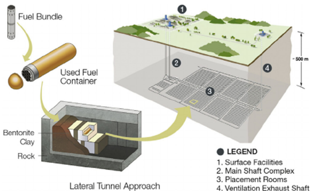
Figure 3.1-3. NWMO's Mark II concept (Boyle and Meguid 2015).
