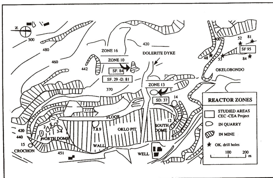
Figure 11.1-1. A map of the reactor zones in the Oklo area (Hollinger 1992).
