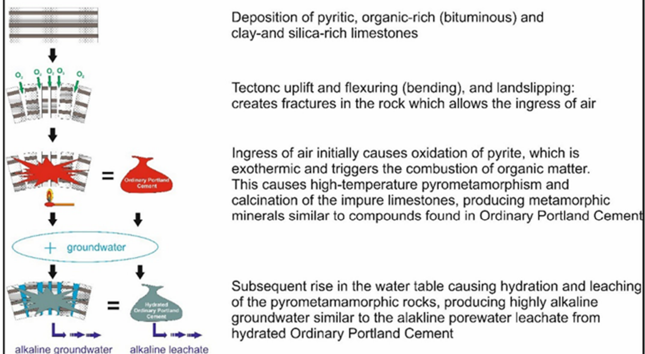
Figure 4.1.3-2. Schematic representation of the production of the natural concretes at Maqarin (Alexander et al. 2005).
