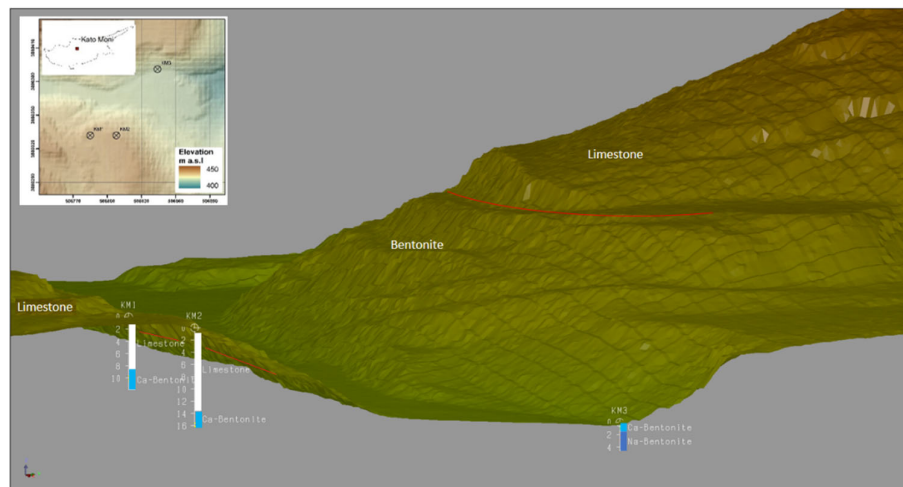
Figure 5.1.3-3. 3D model of the Kato Moni (Cyprus) quarry topography (view looking to the NW). Boreholes KM1-KM3 (depths shown in meters) with KM1 and KM2 drilled through limestone (white) into the bentonite (blue) beneath and KM3 drilled straight into bentonite (blue colours). Red line shows the bentonite - limestone boundary at the northern and southern hill slopes (modified from Reijonen et al. 2017).
