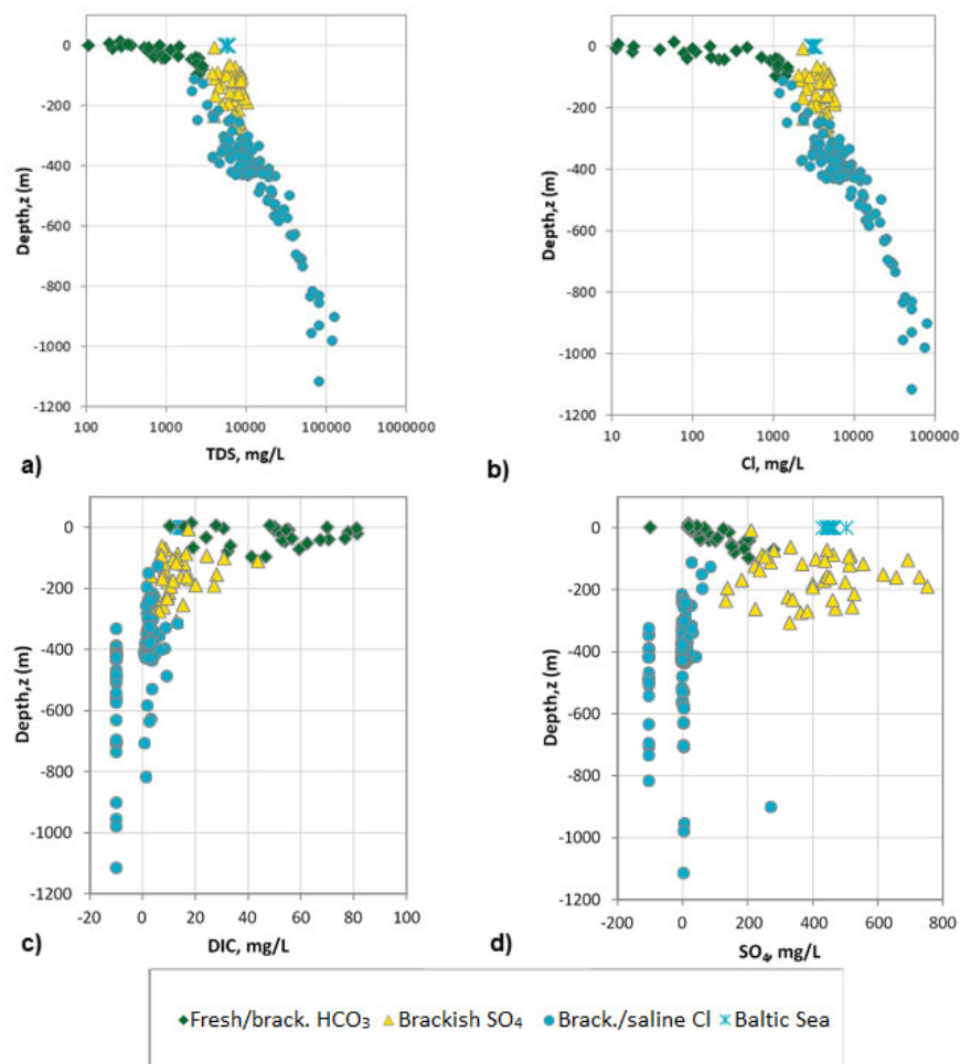
Figure 6.2.1-3. a) TDS, b) Cl, c) DIC and d) SO 4 concentrations of Olkiluoto baseline 6 groundwater samples as a function of depth. Negative values in c) and d) indicate results below detection limit. Note, a logarithmic scale is used for TDS and Cl, whereas a linear scale is used for DIC and SO 4 . Posiva (2022).
