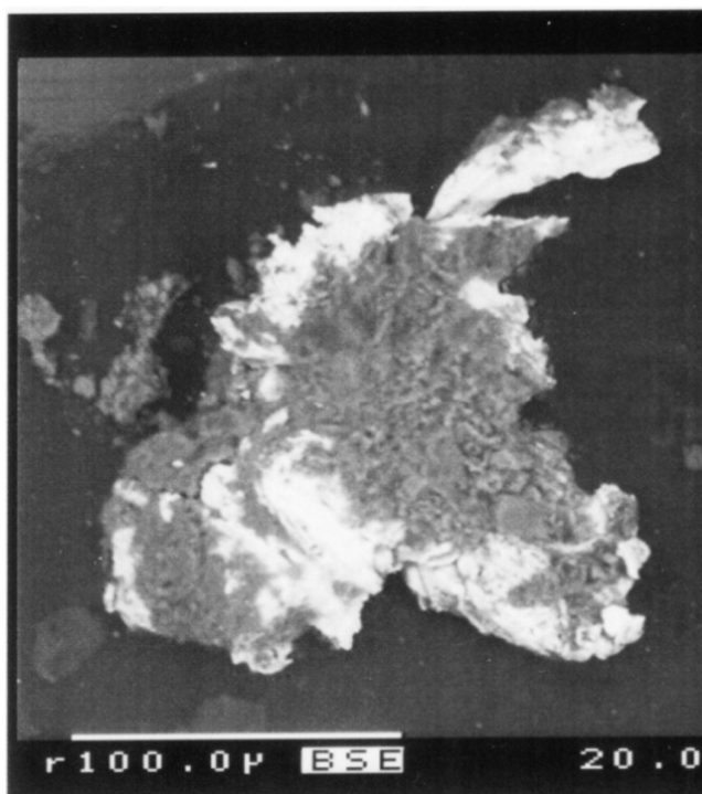
Figure 3.1.2-2. Native copper plate (white) covered with smectite (gray mass in the middle) from a groundwater conducting fracture at Hyrkkölä, SW Finland (Marcos 2002)
