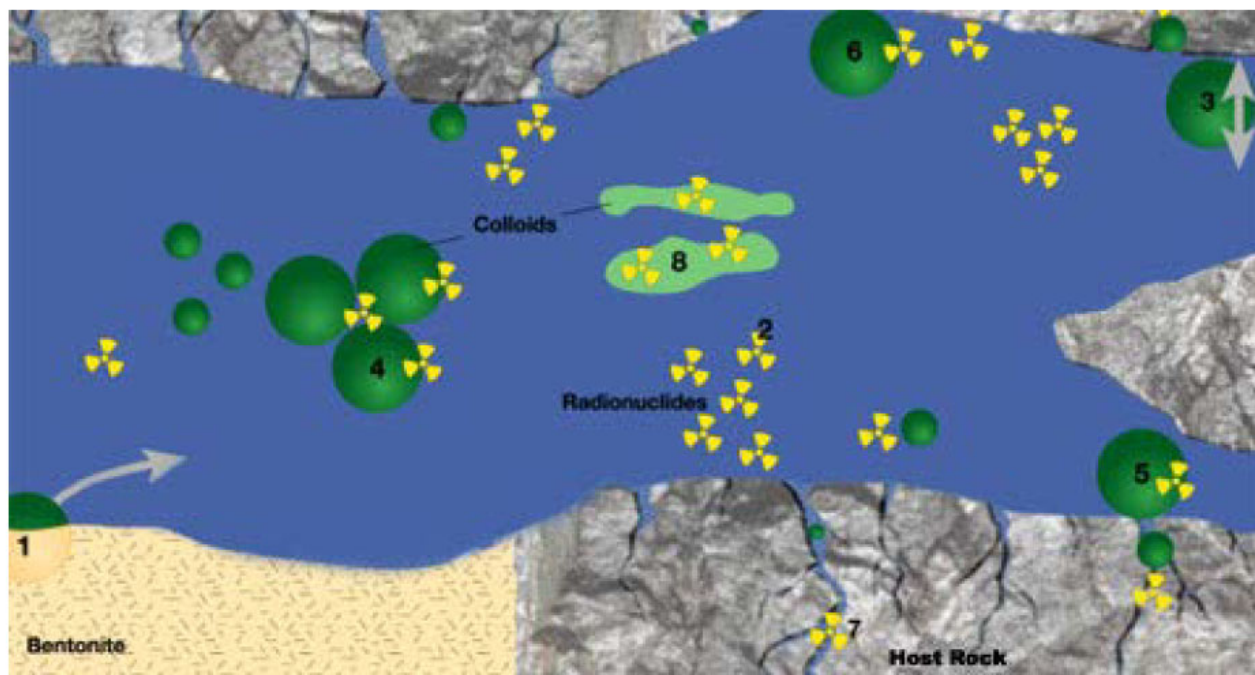
Figure 8.3-1. Potential production mechanisms of colloids (for example at the bentonite barrier/host rock interface) and subsequent transport of radionuclides in fractures in the host rock (Image courtesy of Nagra).
