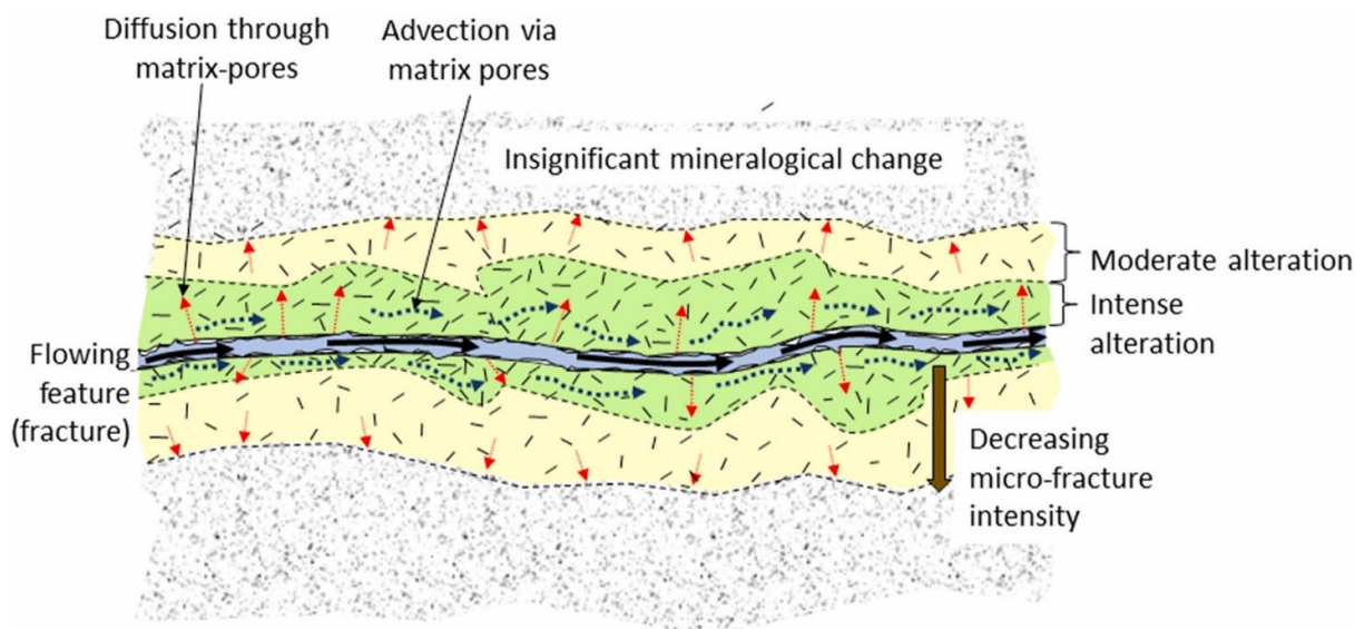
Figure 8.4-1: Conceptual model for radionuclide uptake in a fractured GDF host rock (Metcalf et al. 2021)
