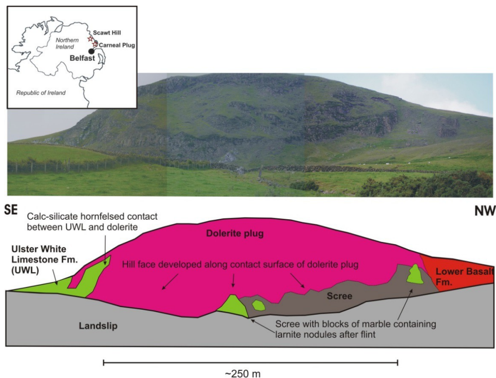
Figure 4.1.4-1. Location of the natural analogue study sites and a simplified geological cross-section of Scawt Hill (from Milodowski et al. 2011).
