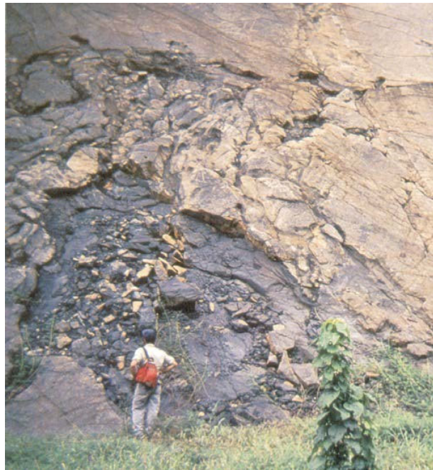
Figure 2.2.1-2. Imprint of the core of a natural reactor on the pit wall at Oklo (Miller et al. 2000).
