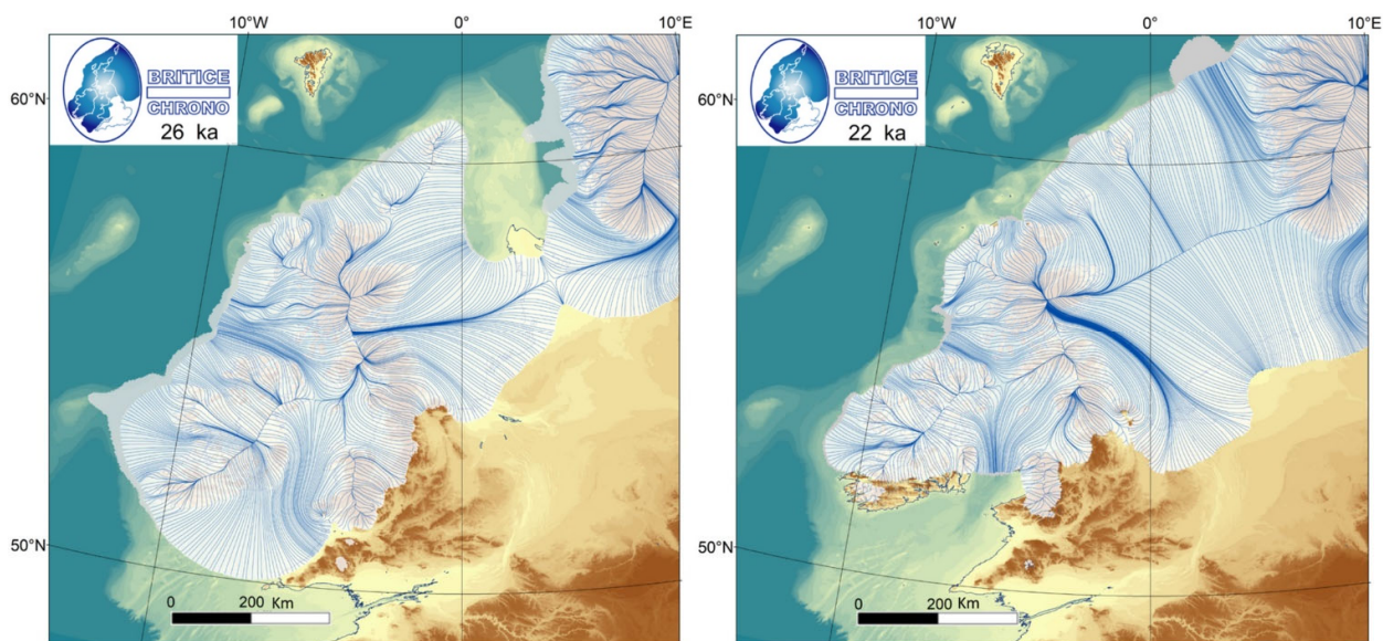
Figure 7.1-2. Ice-sheet extent and flow geometry (ice shelves in grey) at the maximum areal extent of the British–Irish Ice Sheet (left panel; 26 ka) and North Sea Ice Sheet (right panel; 22 ka). Build-up of ice over the North Sea occurred by head-on collision of British and Scandinavian ice lobes (left panel; 26 ka) resulting in an ice saddle that rapidly grew in elevation to build the major North Sea Ice Divide (1500 m thick) by 22 ka. Clark et al. (2022)
