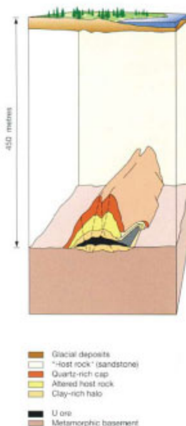
Figure 2.1.2-1. Cross-section of the Cigar Lake orebody (after Miller et al. 2000)
