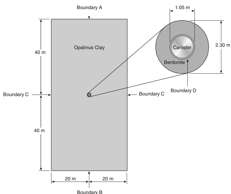
Figure 1. Conceptual model for the calculation of glacially-induced flow and transport in bentonite and Opalinus Clay (Nagra, 2002c)
