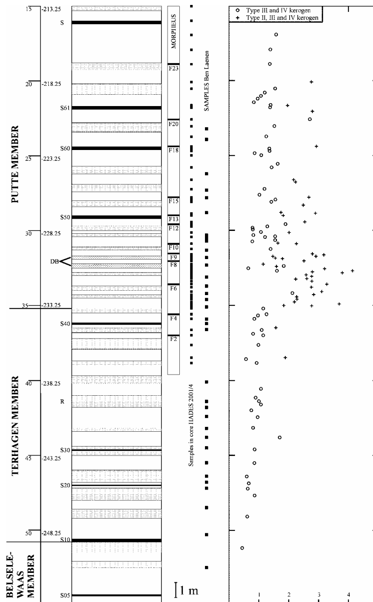
Figure 1. On the left the analysed Boom Clay stratigraphy is given together with the depth to the URF and the depth to Second General Leveling in Belgium. On the right the TOC content in function of depth is given.
