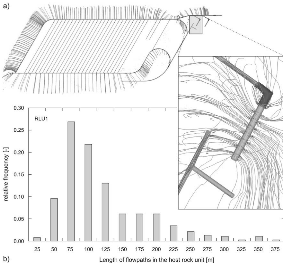
Figure 1. Expulsion of porewater from the disposal areas of an SF/HLW/ILW repository that may be caused by glacial loading (Kuhlmann & Marschall 2003) (a) flow patterns and (b) length of flow paths in the host rock formation (ILW disposal tunnel)
