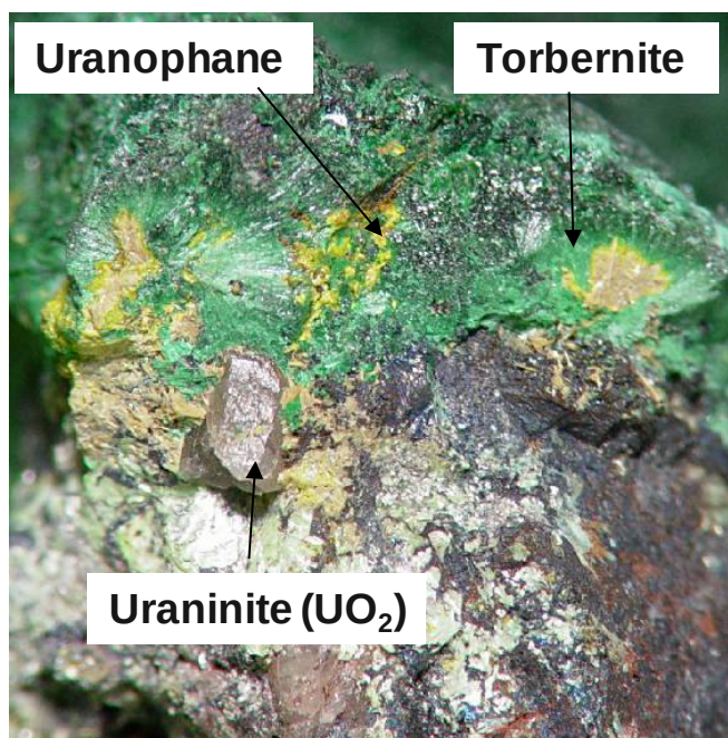
Figure 6. Uraninite is altering to secondary uranium minerals torbernite ( \text{Cu}(\text{UO}_2)_2(\text{PO}_4)_2 \cdot 12\text{H}_2\text{O} ) followed by uranophane ( \text{Ca}(\text{UO}_2)_2[\text{HSiO}_4]_2 \cdot 5\text{H}_2\text{O} ).
