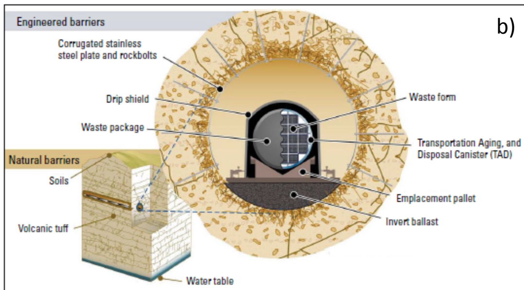
Figure 1. a) Photograph of the Yucca Mountain Project (YMP) site and b) image showing the engineered and natural barriers associated with the YMP DGR concept. Images are from Wikipedia and USGS (2010), respectively.
