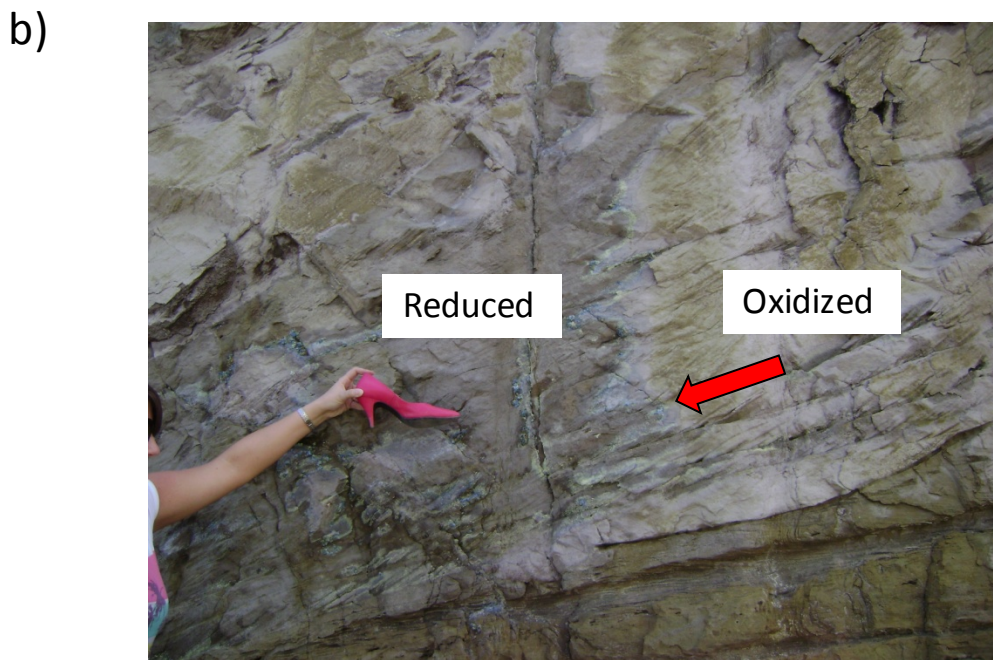
Figure 7. a) A schematic representation of a roll-front uranium deposit showing the complex structure of the ore zone, and b) an outcrop of a roll-front deposit, Turkey Creek, Colorado, USA show the reduce (grey) and oxidized zones (beige/light grey).
