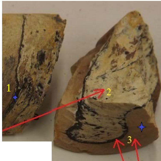
Figure 4. Image of a core samples from the End uranium deposit, Kiggavik area, Nunavut, Canada. Area 1 shows uranium minerals along a fracture, and areas 2 and 3 show secondary uranium mineralization within a clay rich matrix.
