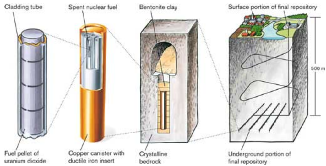
Figure 5. Cartoon illustration of used nuclear fuel pellets within a fuel assembly, waste package and DGR environment. Image is from IAEA (2012).
